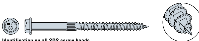
Identification on all SDS screw heads
