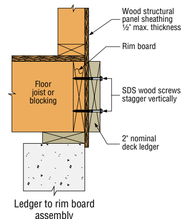
Ledger may not be installed over siding or stucco. It must be fastened directly to the rim joist or sheathing.
