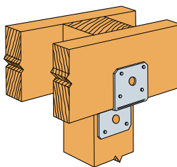
DJT: Connects beams at the side of the post.
